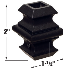
9064AK-* \frac{1}{2} Adjustable Knuckle 50 pcs per box
